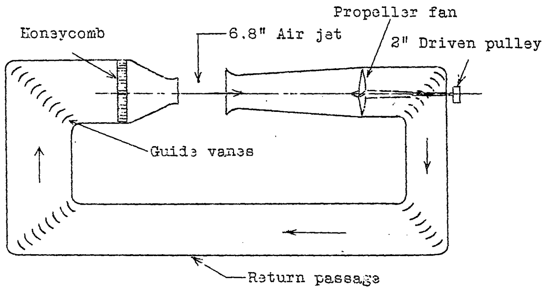
Fig.2 Six Inch Wind Tunnel With Propeller Fan
