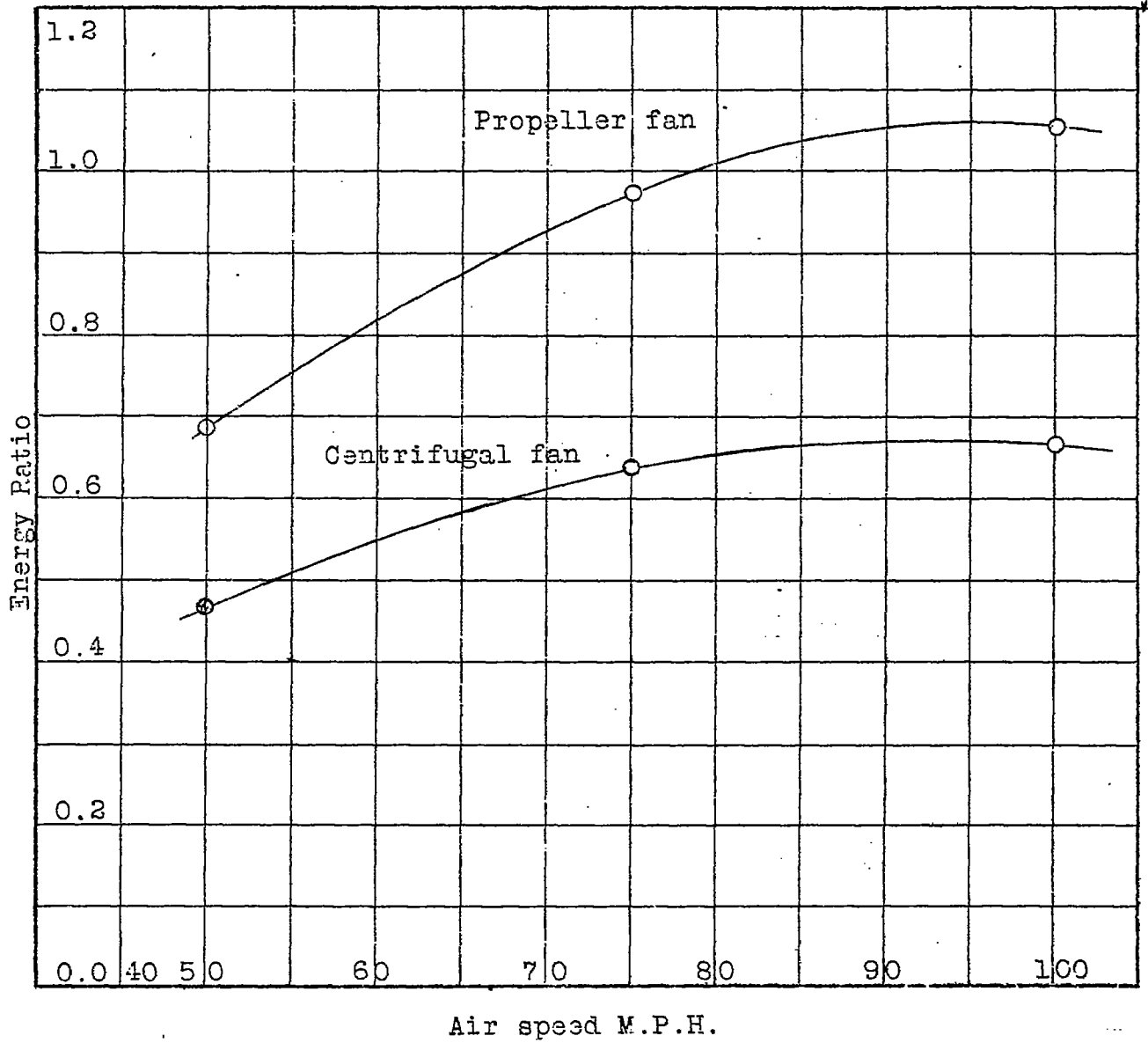
Fig.4 Energy Ratio of N.A.C.A. Six Inch Wind Tunnel With Propeller Fan and With Centrifugal Fan.
